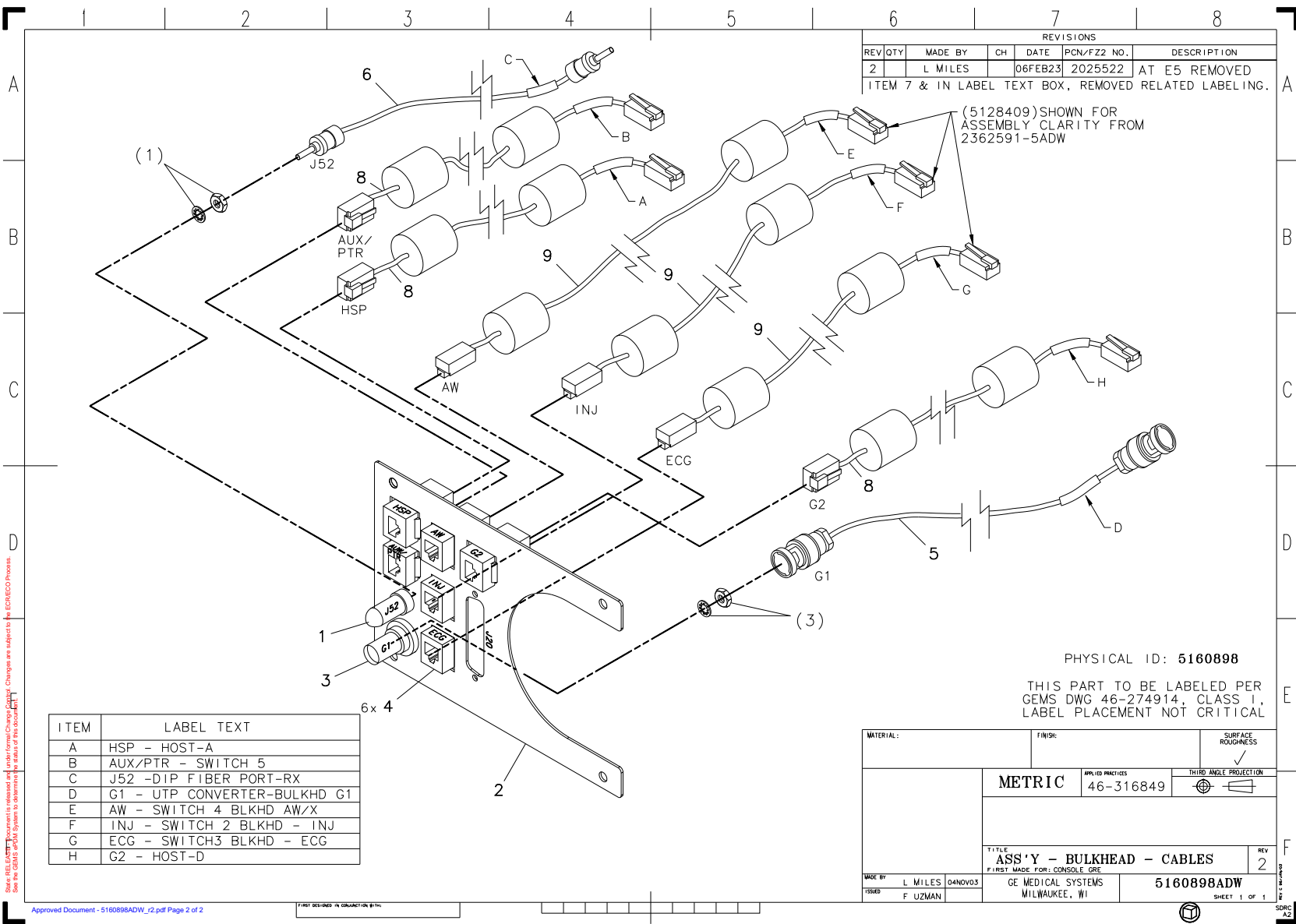
Figure 5-17 SubAssy, GRE Console Rear Bulkhead (5160898ADW, Rev 2)
