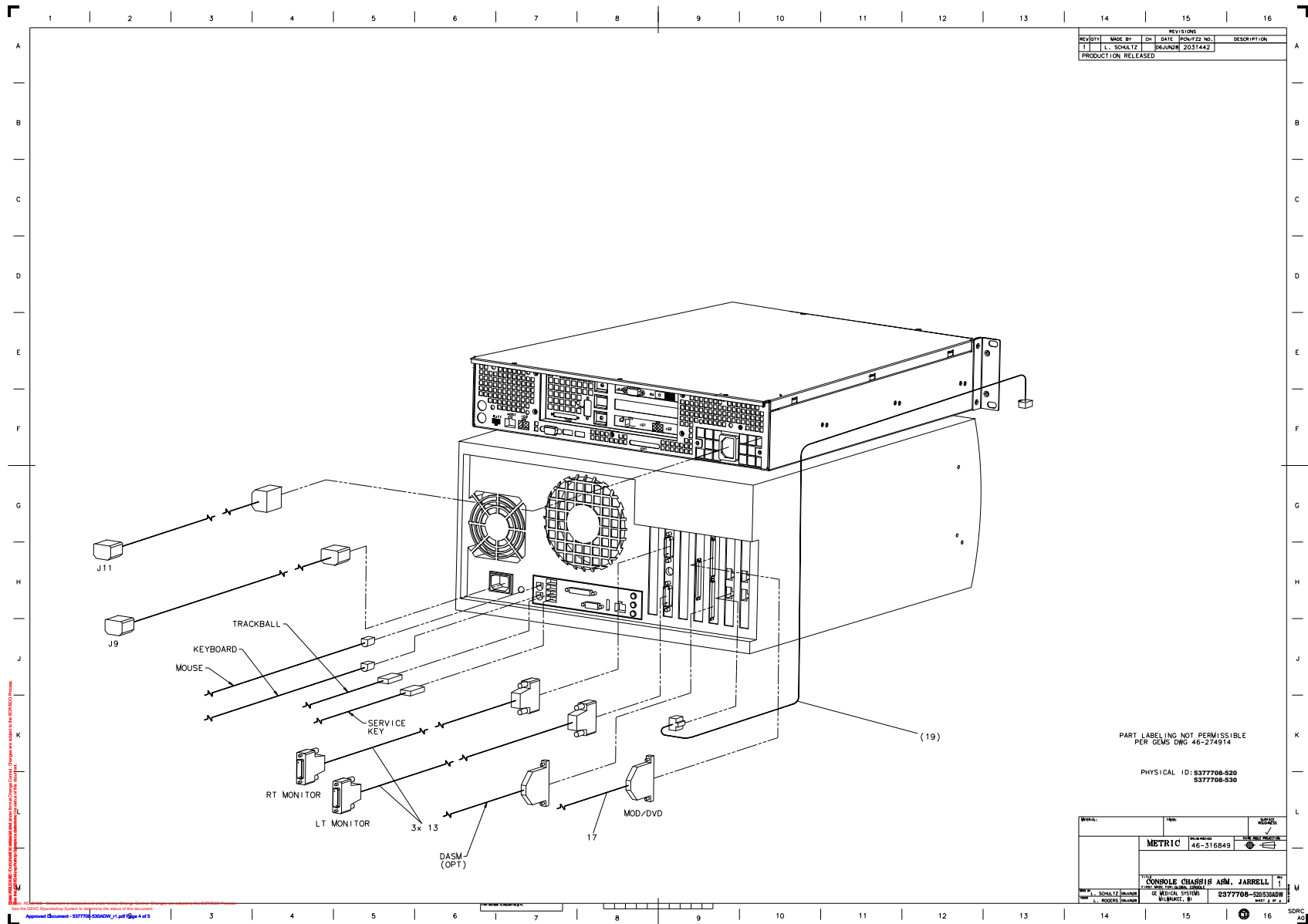
Figure 5-13 GRE Console, 16 Slice Gdas For Bs With Xw8200, Ethernet Switch And Jarrell (5377708-530ADW, Sheet 3, Rev 1)
