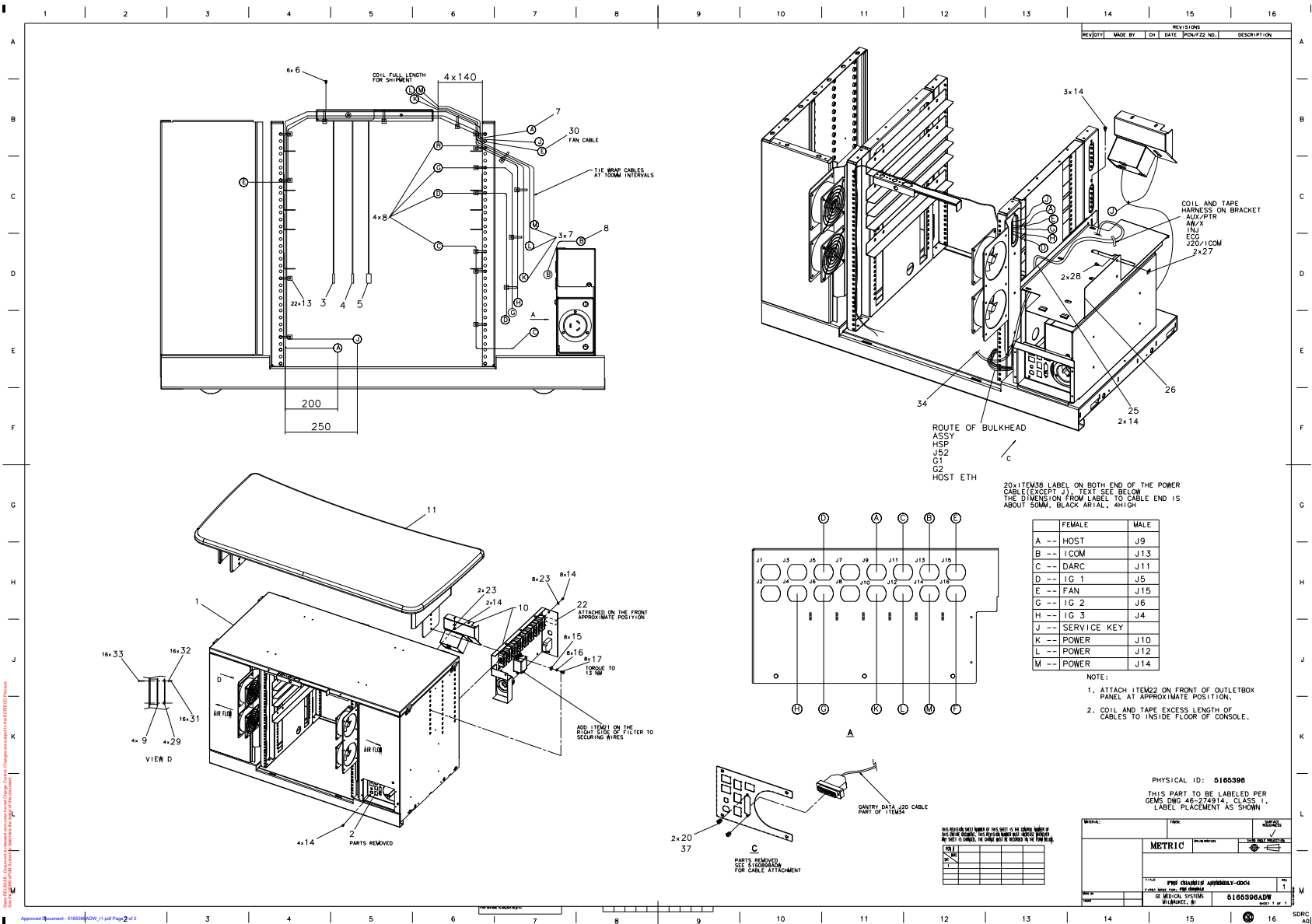
Figure 5-15 FWS GOC4 Chassis Assembly (5165396ADW, Sheet 1, Rev 1)
