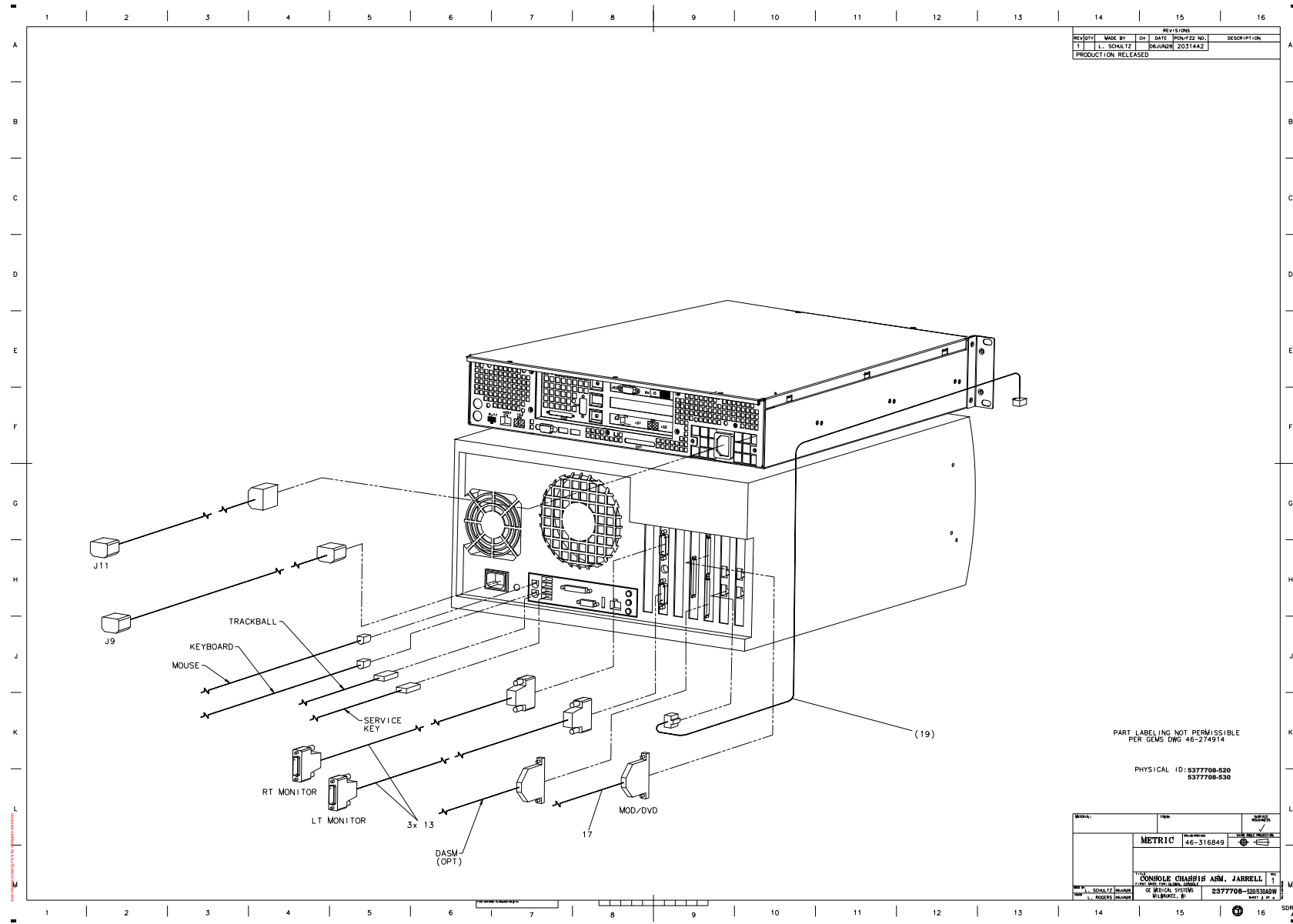
Figure 5-25 GRE Console, 4/8 Slice GDAS for BS with XW8200, Ethernet Switch and Jarrell (5377708-520ADW, Sheet 3, Rev 1)
