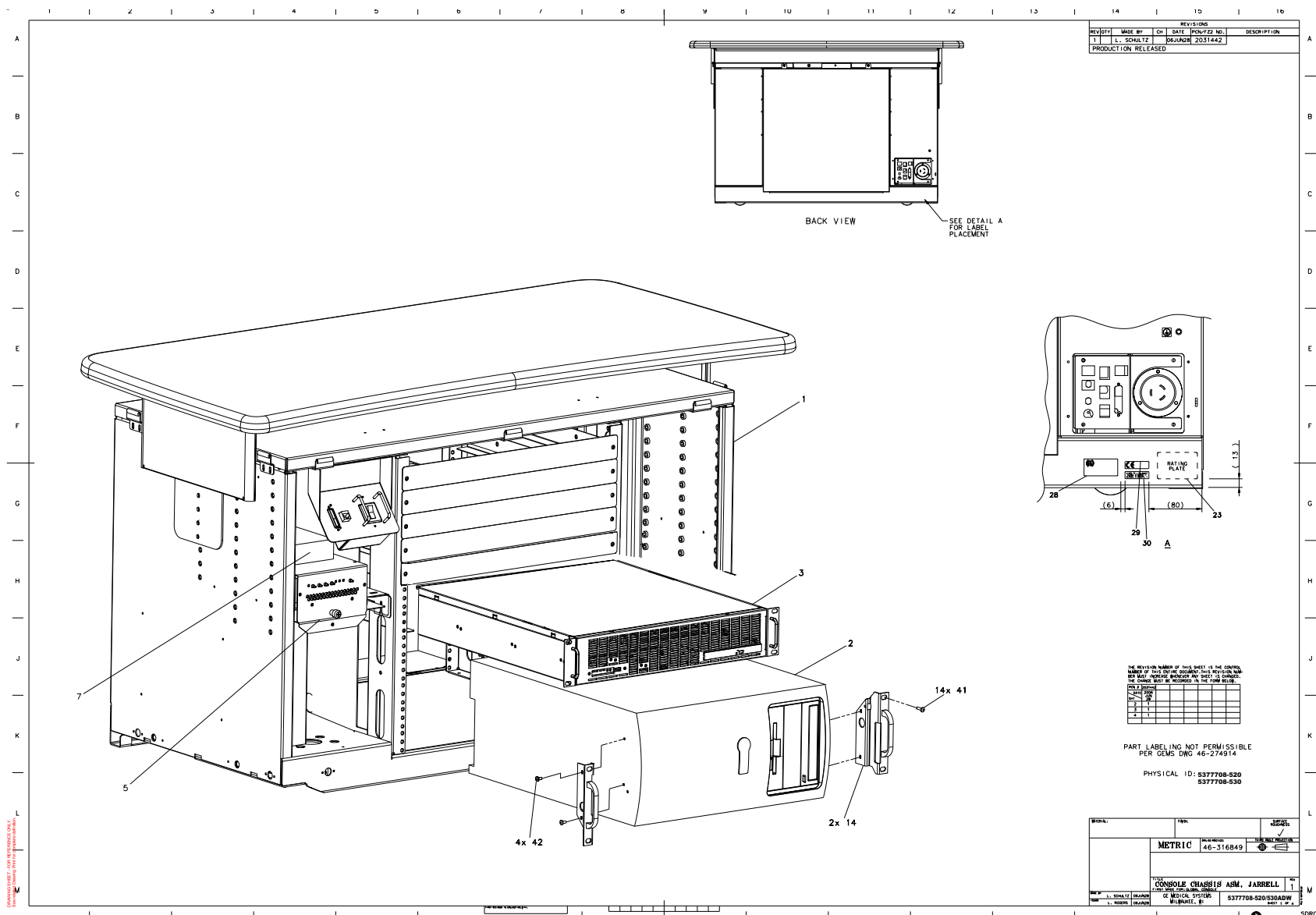
Figure 5-23 GRE Console, 4/8 Slice GDAS for BS with XW8200, Ethernet Switch and Jarrell (5377708-520ADW, Sheet 1, Rev 1)
