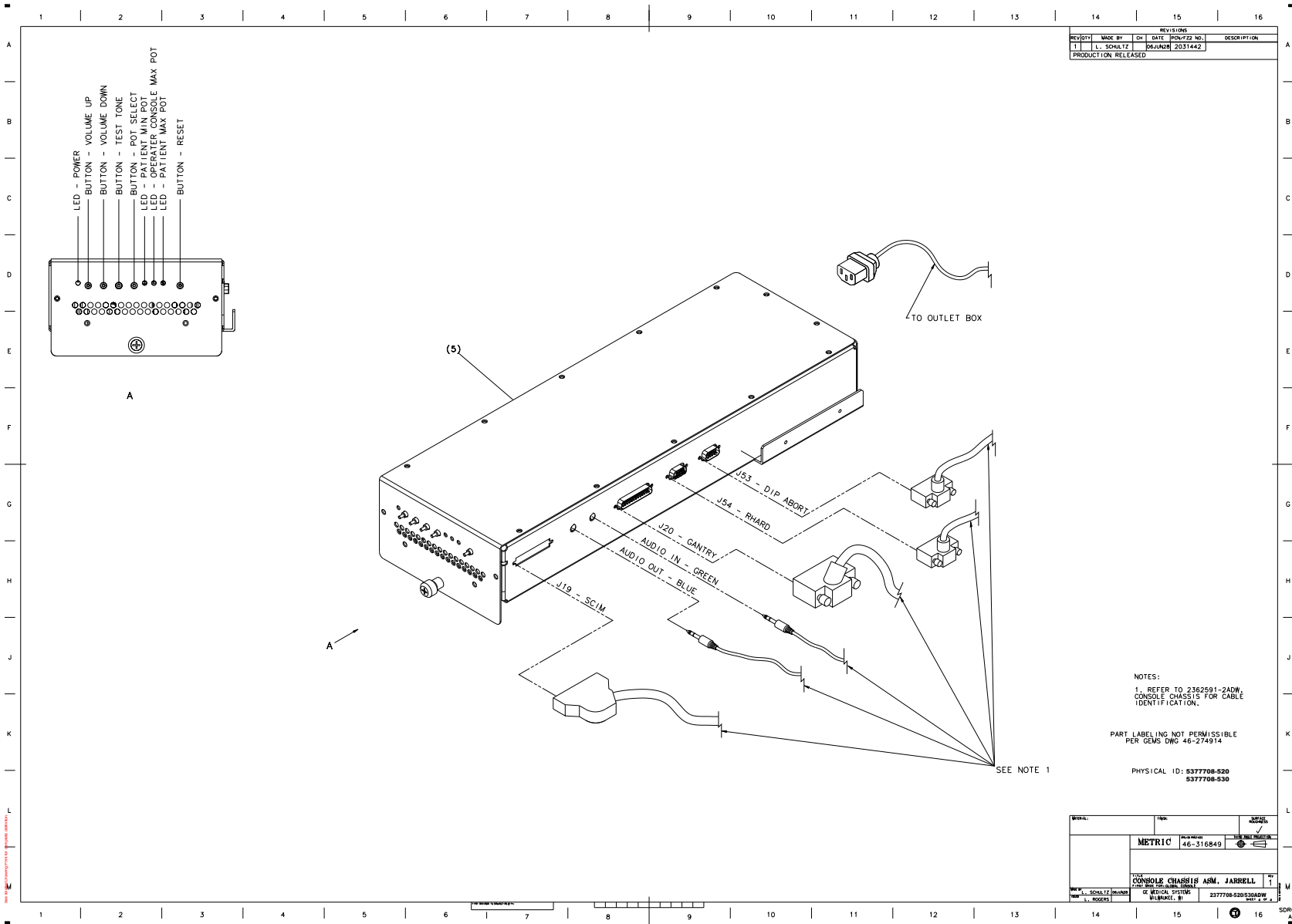
Figure 5-26 GRE Console, 4/8 Slice GDAS for BS with XW8200, Ethernet Switch and Jarrell (5377708-520ADW, Sheet 4, Rev 1)
