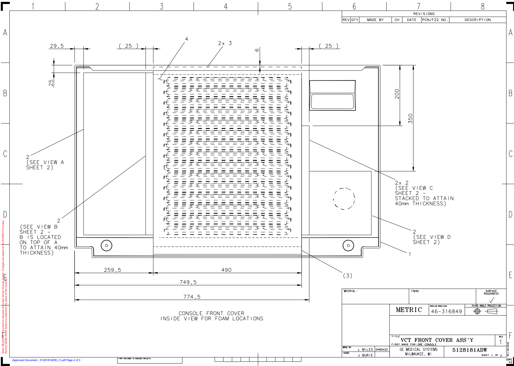
Figure 5-21 Cover Assy - Console Front (5128181ADW Sheet 1, Rev 1)
