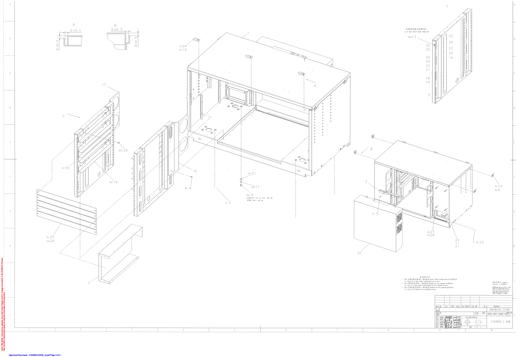
Figure 5-6 FWS GOC4 chassis (5164805-2ADW, Sheet1, Rev2)
